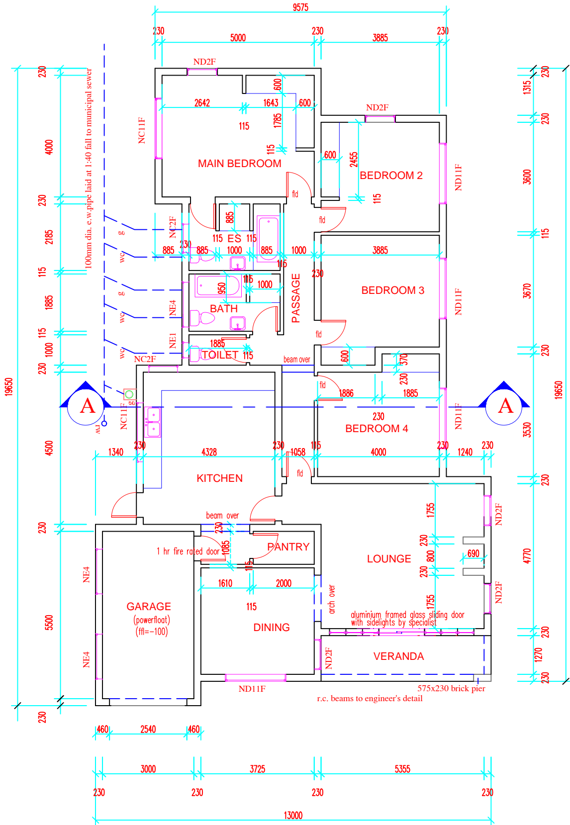
FLOOR PLAN 1:100 (206sqm)
